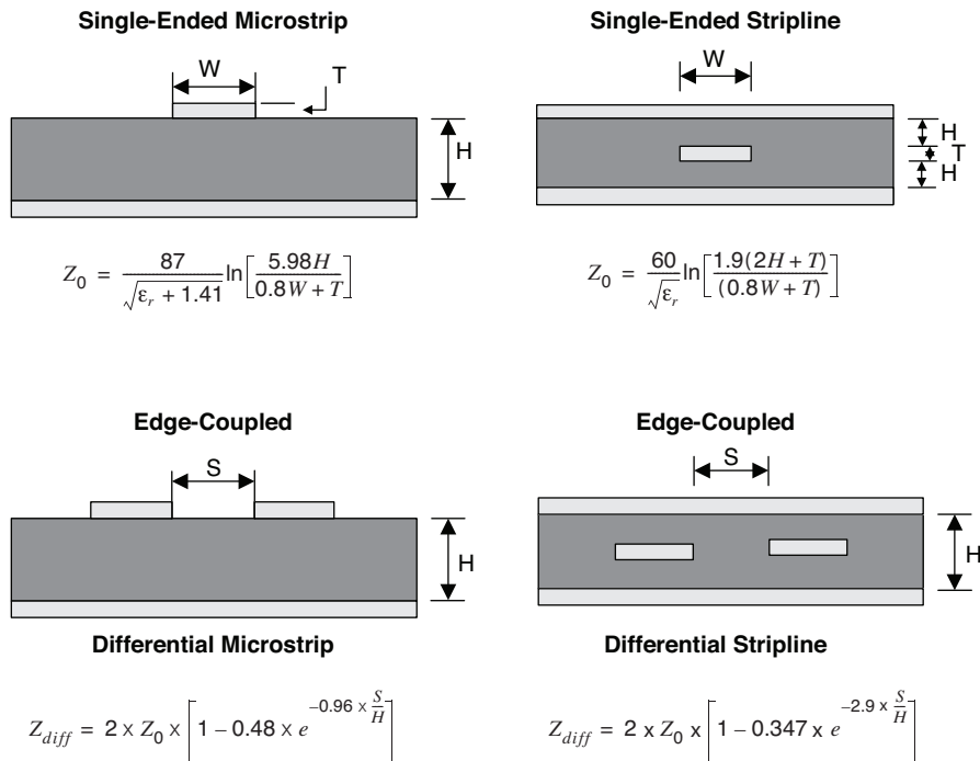
Figure 6. Controlled Impedance Transmission Lines
