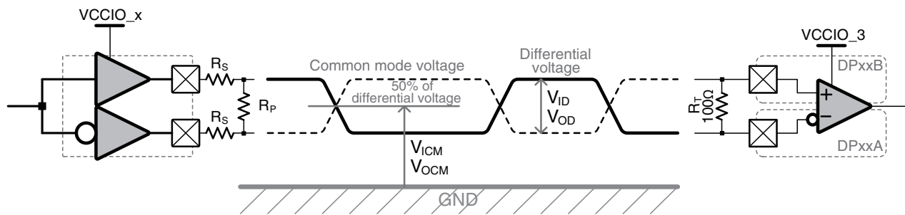
Figure 1. Differential Signaling Electrical Parameters
