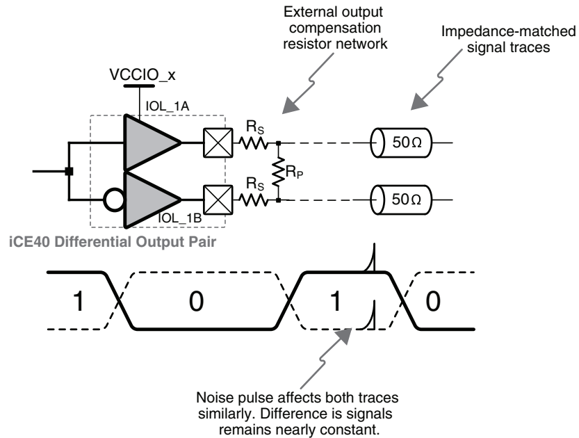
Figure 2. Differential Output Pair
