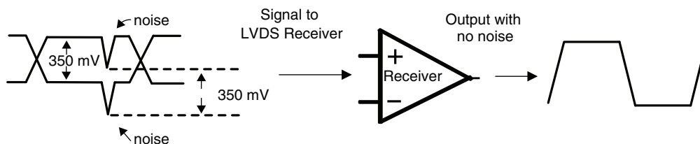
Figure 8. Differential Input Eliminates Common-Mode Noise
