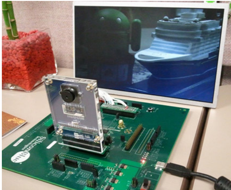
Figure 12. 5-Megapixel CMOS Camera to LVDS Display on iCEman40 Evaluation Board
