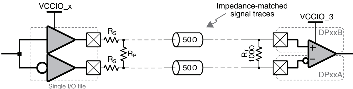
Figure 3. iCE40 LVDS or Sub-LVDS Differential I/O Channel
