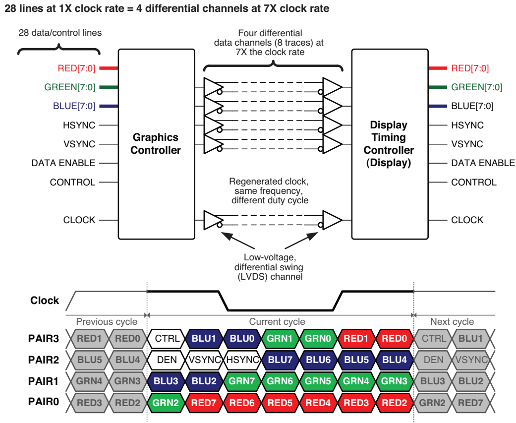
Figure 11. Example Differential I/O Solution: Flat Panel Display Interface
