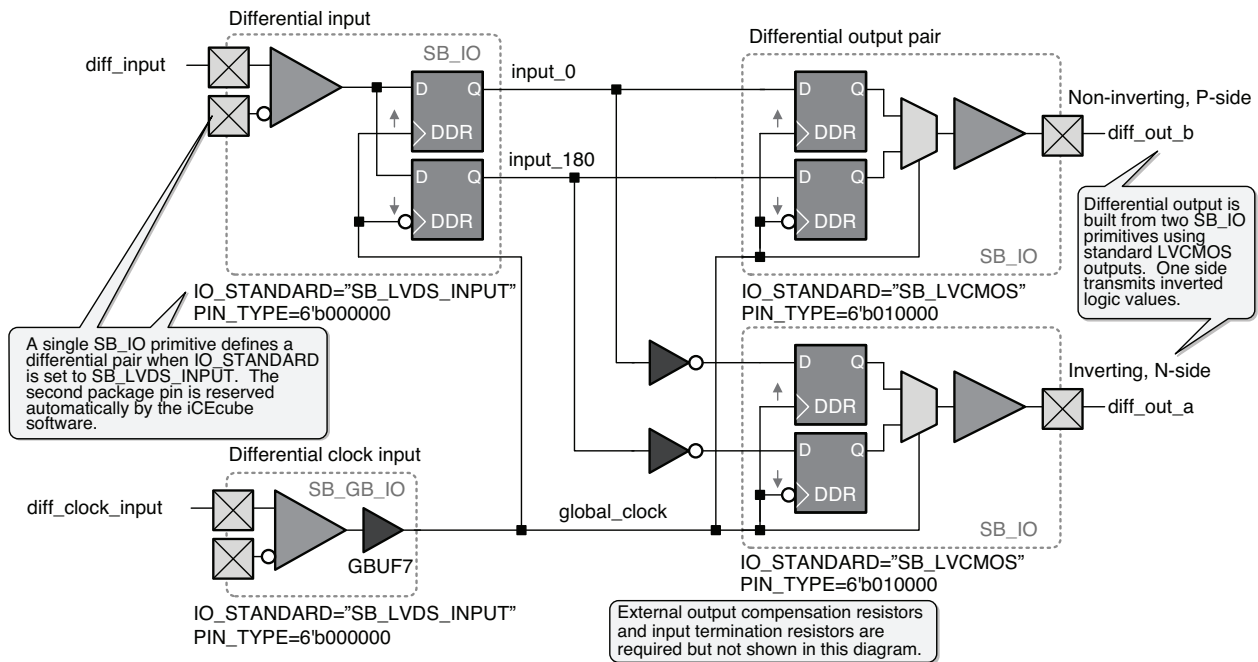
Figure 9. Differential I/O Design Example
